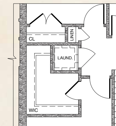
OPT. SECOND FLOOR LAUNDRY
