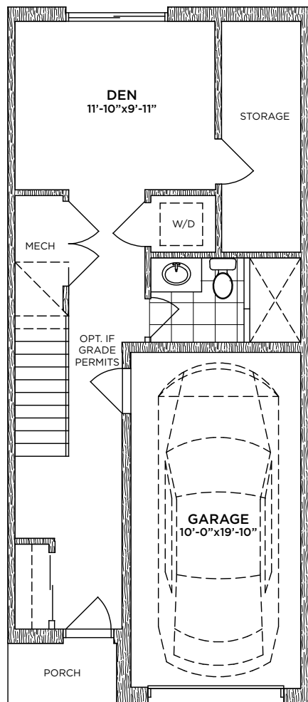
GROUND FLOOR B STANDARD
