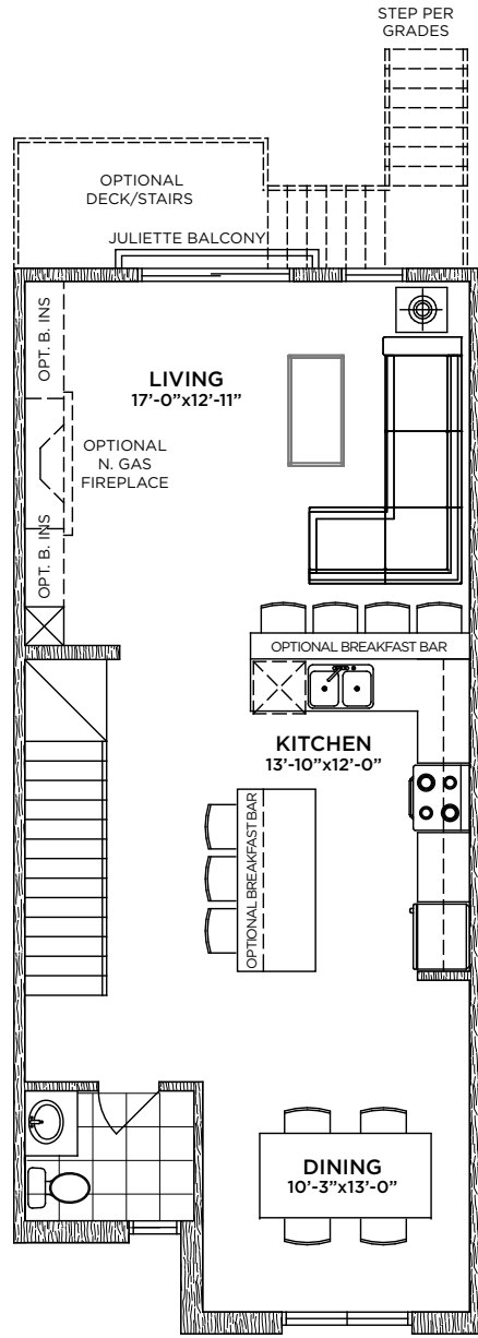
END UNIT WITH GARAGE ON EXTERIOR SIDE OF BUILDING
