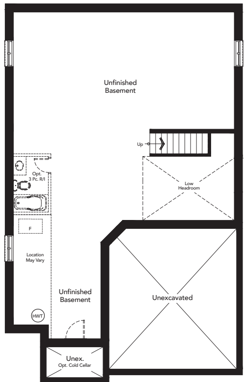
BASEMENT Elev. A
