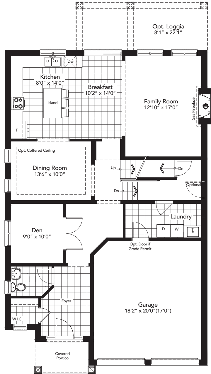
ALT. GROUND FLOOR Elev. A
