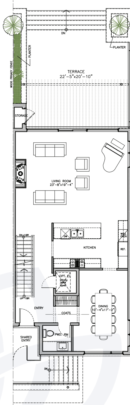
FIRST FLOOR
